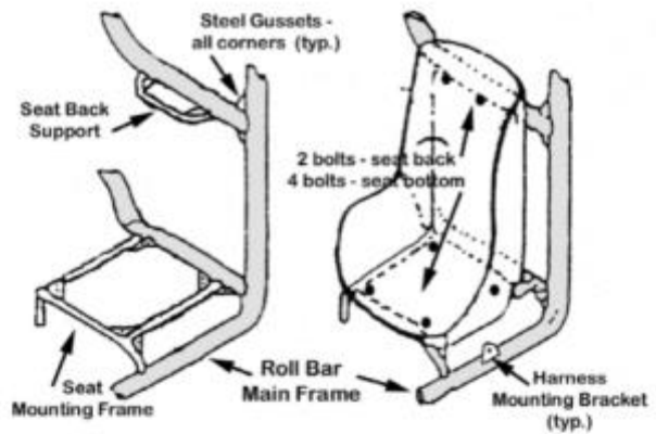
Basic Seat Installation
